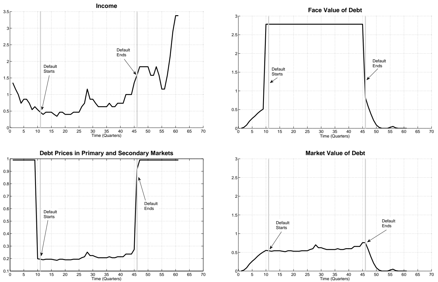
Figure 4: Simulation of i.i.d. Creditor Example
