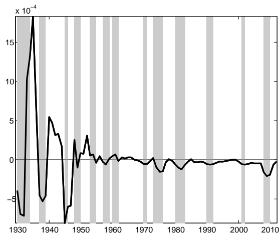
Fig. 2. Residual positive variance. The figure shows the time series plot of the residual positive variance, smoothed over a 3-year window, which is orthogonal to the negative variance. The positive and negative realized semivariances decompose the total realized variance into the components pertaining only to positive and negative movements in industrial production growth, respectively. The residual positive variance is computed from the projection of the positive realized semivariance onto the negative one. The shaded areas represent NBER recessions.
