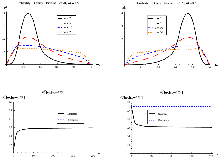
Figure 2: Top panel: the probability density function of \omega_u given a current value of \omega_t = 0.25 (left-hand side) and \omega_t = 0.75 (right-hand side). Bottom panel: expected values of the same.
