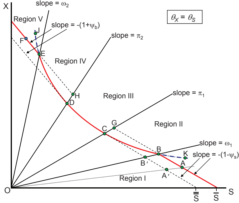
FIGURE 1: Indifference Curve of the Value Function When \theta_X = \theta_S .
