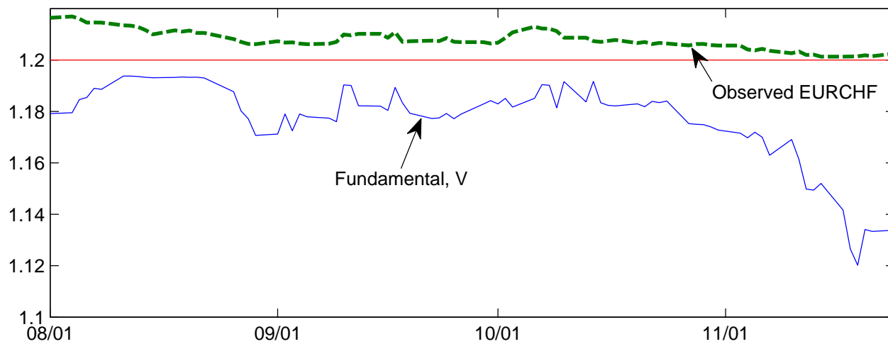
Observed and fundamental exchange rate CHF per EUR
